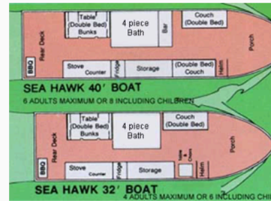
40' SEAHAWK LAYOUT
